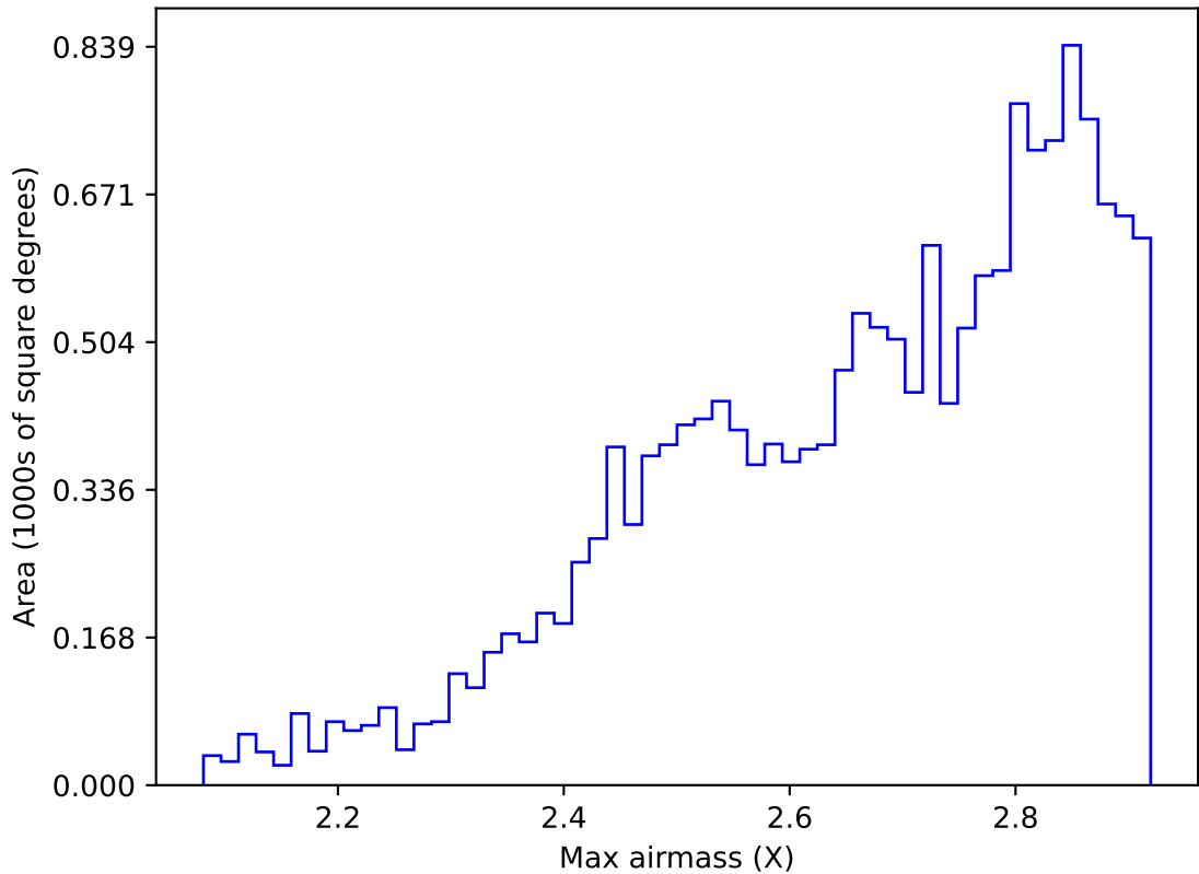
too_elab_r16_d3_griz_v3.4_10yrs WFD all bands: Max airmass
