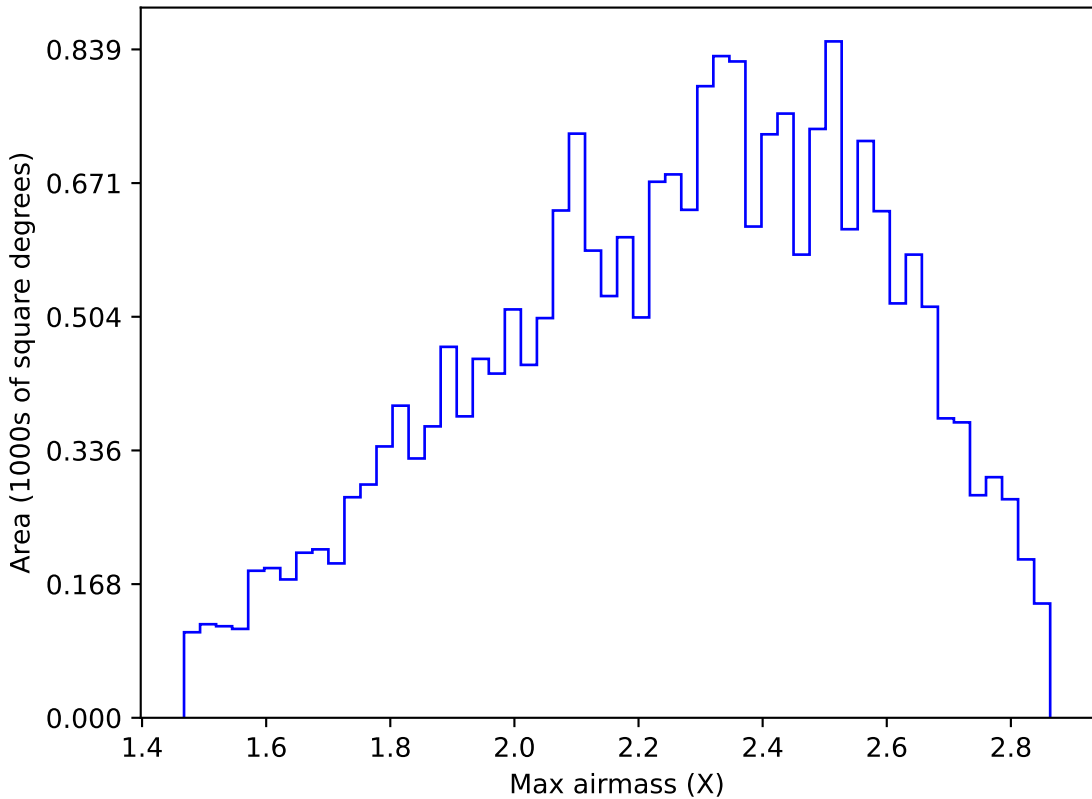
too_elab_r16_d3_griz_v3.4_10yrs All sky y band: Max airmass
