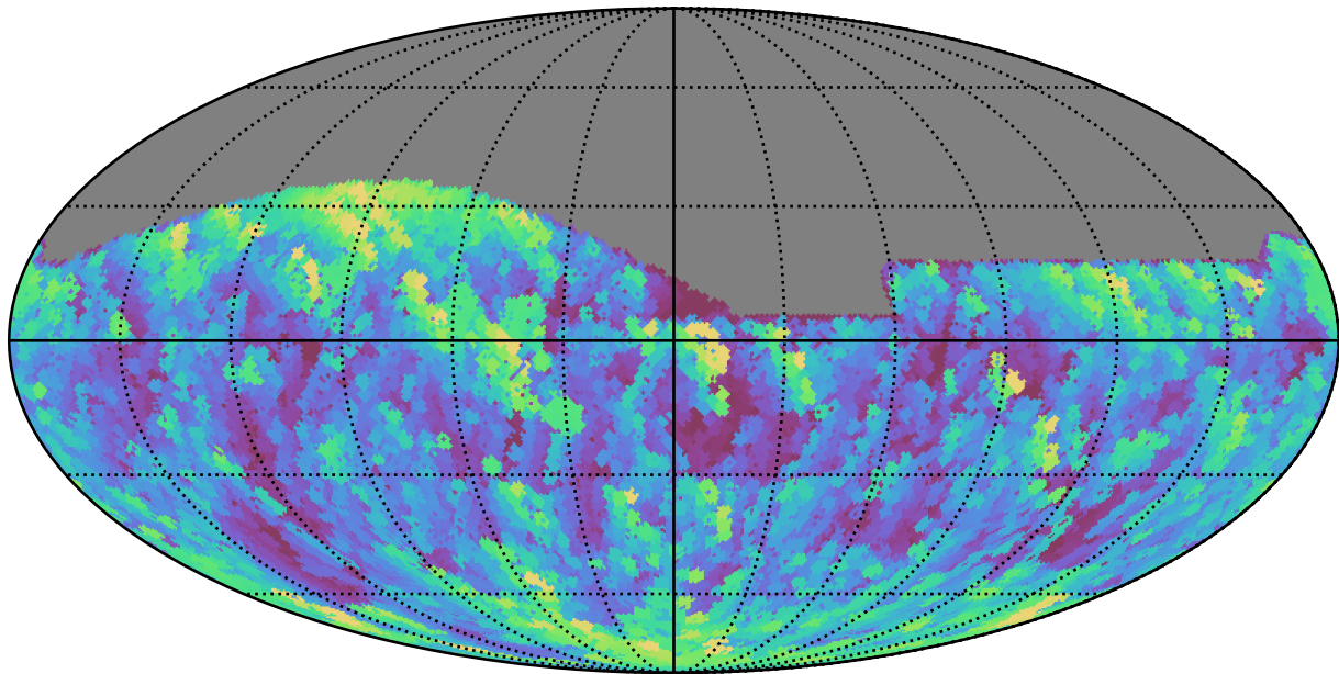
too_elab_r16_d3_griz_v3.4_10yrs All sky g band: Max airmass
