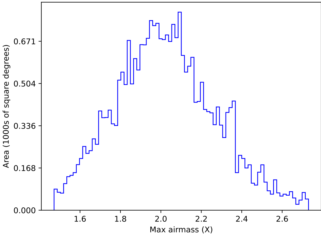
too_elab_r16_d3_griz_v3.4_10yrs All sky g band: Max airmass
