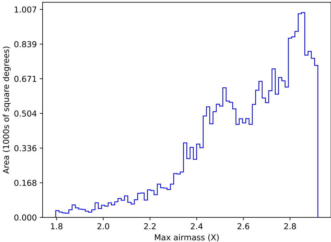
too_elab_r16_d3_griz_v3.4_10yrs All sky all bands: Max airmass
