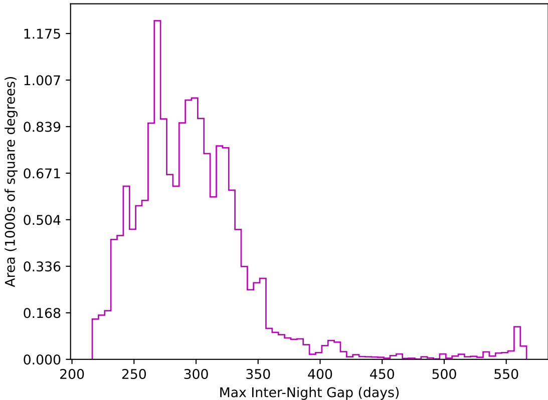
too_elab_r16_d3_griz_v3.4_10yrs WFD z band: Max Inter-Night Gap
