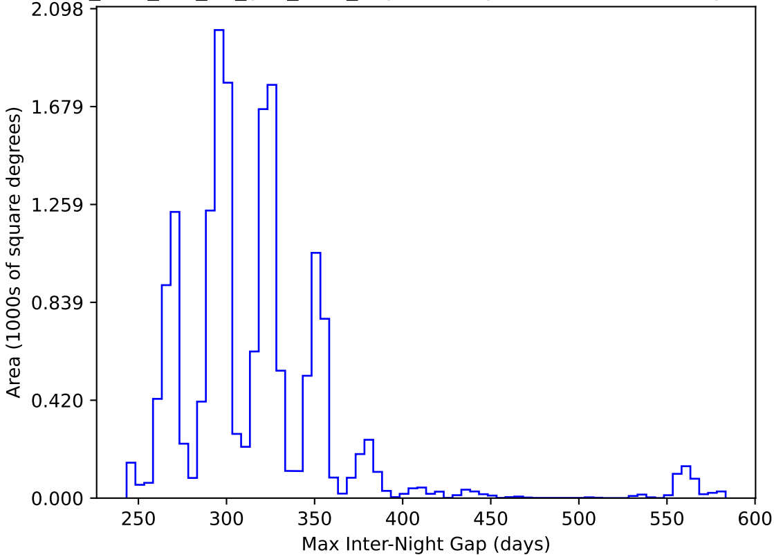
too_elab_r16_d3_griz_v3.4_10yrs WFD y band: Max Inter-Night Gap
