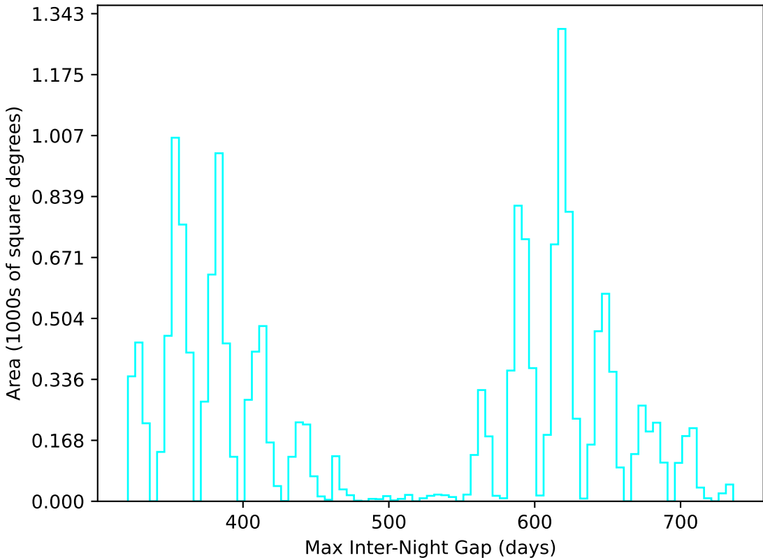
too_elab_r16_d3_griz_v3.4_10yrs WFD u band: Max Inter-Night Gap
