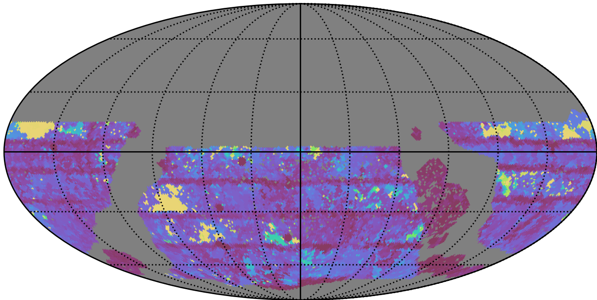
too_elab_r16_d3_griz_v3.4_10yrs WFD i band: Max Inter-Night Gap
