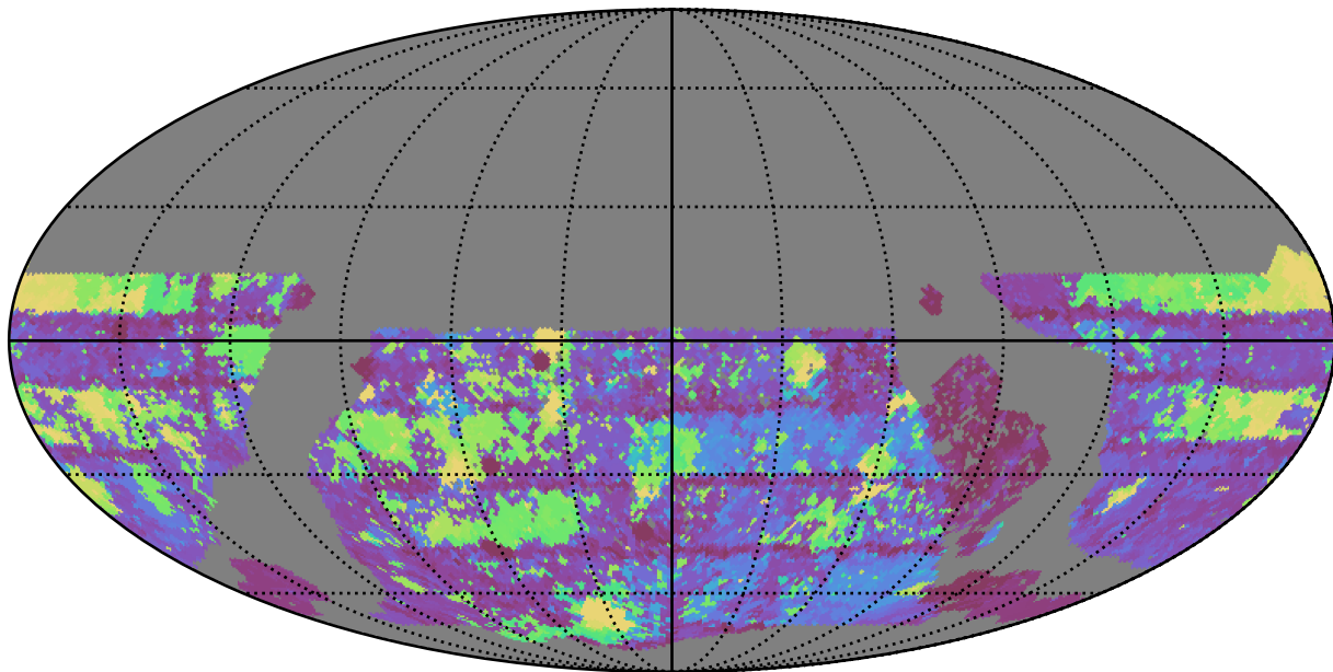
too_elab_r16_d3_griz_v3.4_10yrs WFD g band: Max Inter-Night Gap
