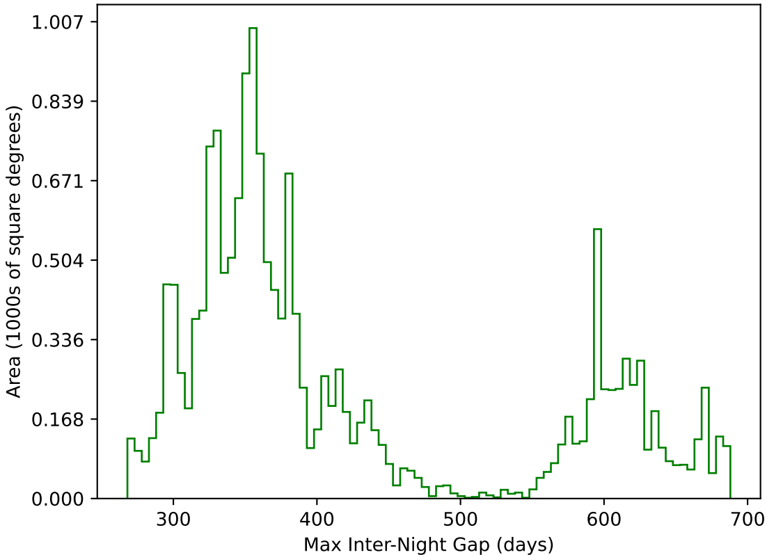
too_elab_r16_d3_griz_v3.4_10yrs WFD g band: Max Inter-Night Gap
