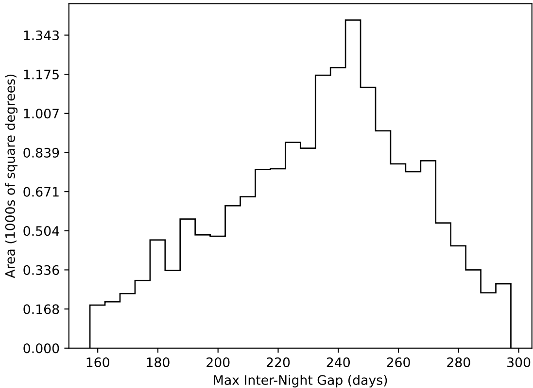
too_elab_r16_d3_griz_v3.4_10yrs WFD all bands: Max Inter-Night Gap
