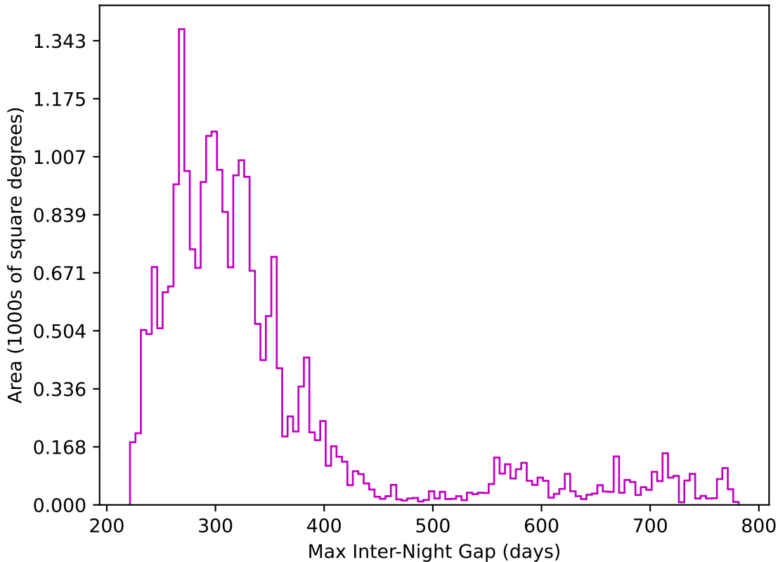
too_elab_r16_d3_griz_v3.4_10yrs All sky z band: Max Inter-Night Gap
