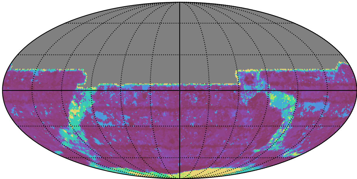
too_elab_r16_d3_griz_v3.4_10yrs All sky y band: Max Inter-Night Gap
