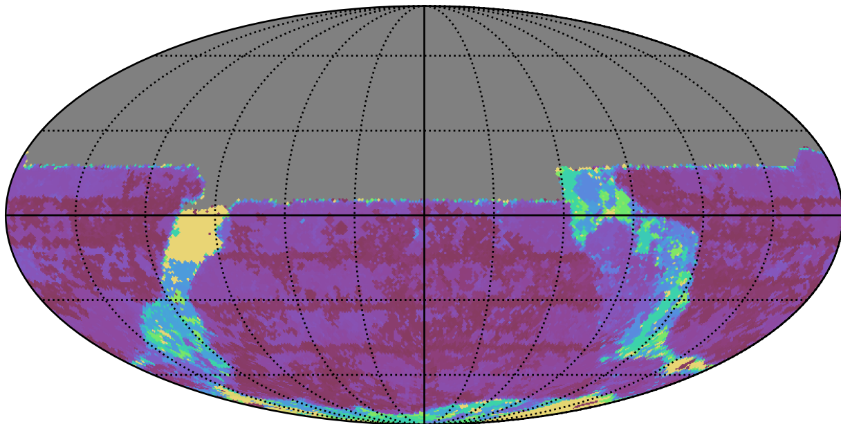
too_elab_r16_d3_griz_v3.4_10yrs All sky u band: Max Inter-Night Gap
