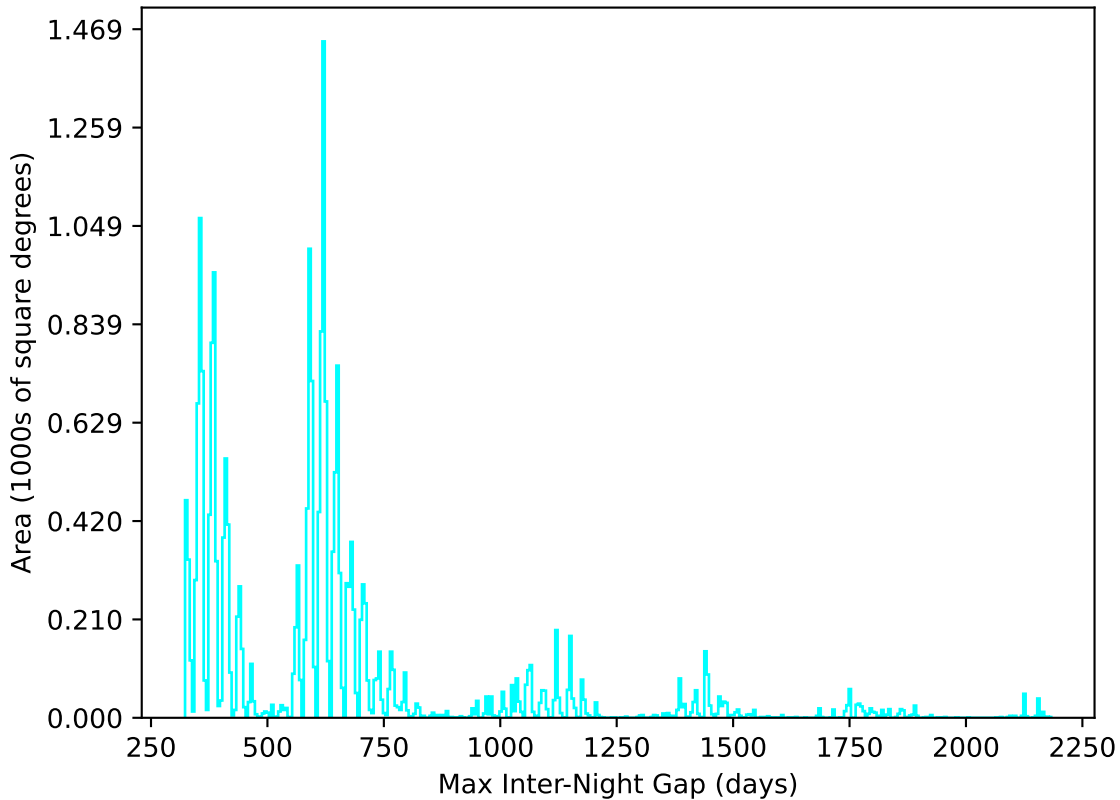
too_elab_r16_d3_griz_v3.4_10yrs All sky u band: Max Inter-Night Gap
