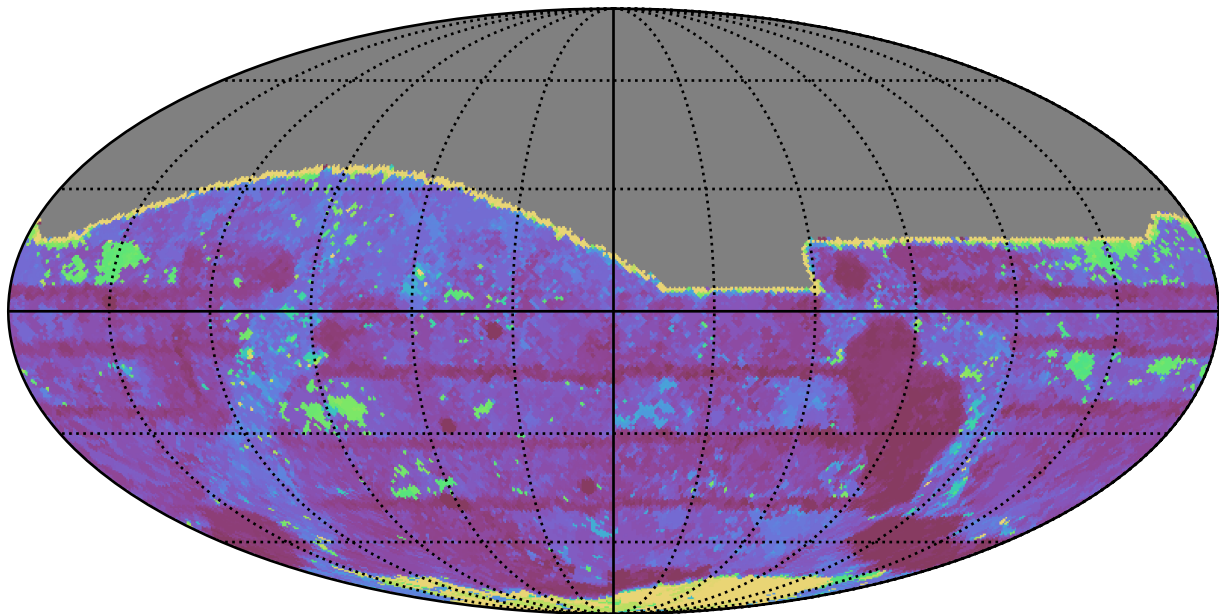
too_elab_r16_d3_griz_v3.4_10yrs All sky r band: Max Inter-Night Gap
