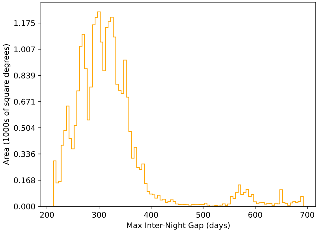
too_elab_r16_d3_griz_v3.4_10yrs All sky r band: Max Inter-Night Gap
