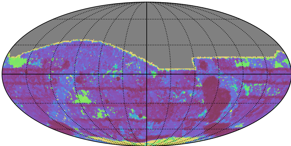
too_elab_r16_d3_griz_v3.4_10yrs All sky i band: Max Inter-Night Gap
