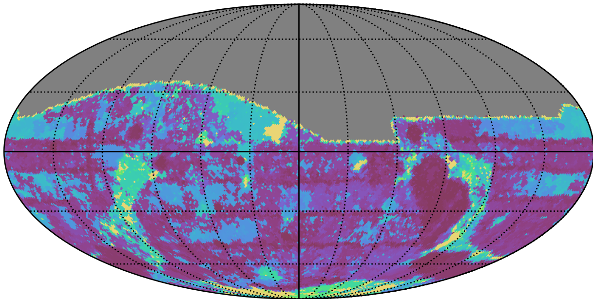
too_elab_r16_d3_griz_v3.4_10yrs All sky g band: Max Inter-Night Gap
