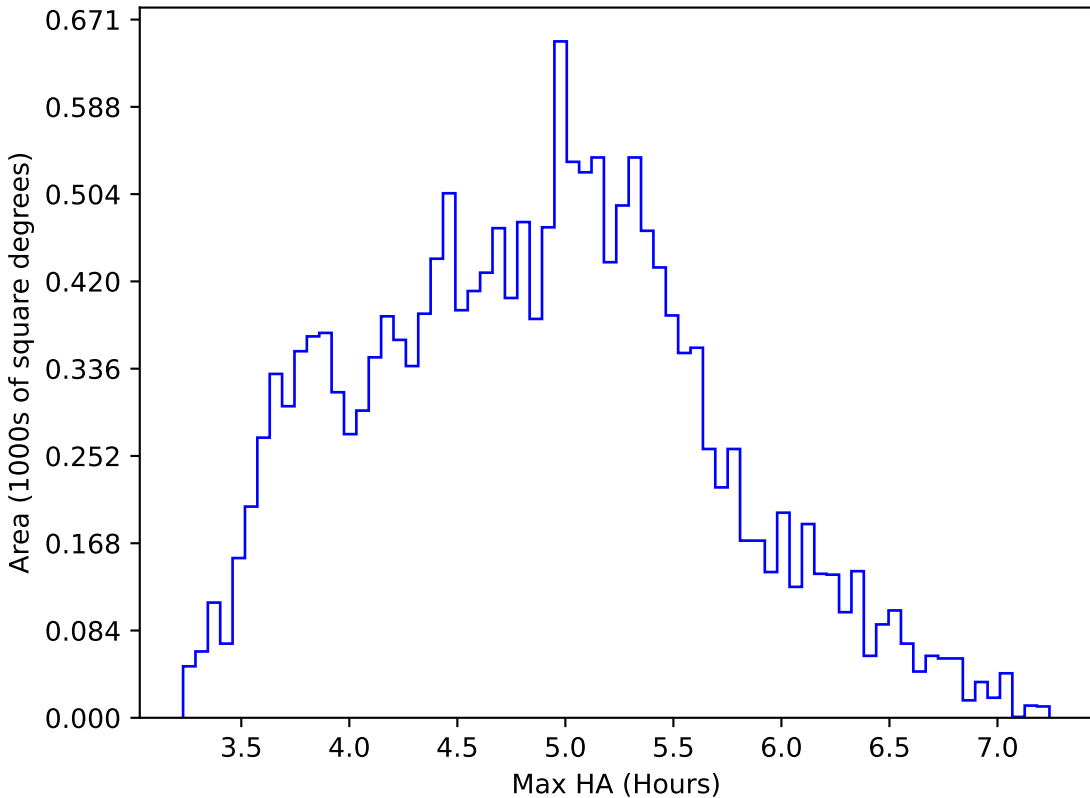
too_elab_r16_d3_griz_v3.4_10yrs WFD z band: Max HA
