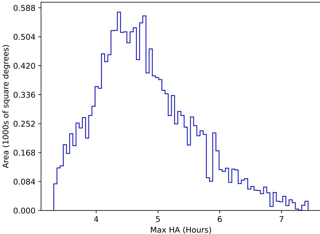
too_elab_r16_d3_griz_v3.4_10yrs WFD y band: Max HA
