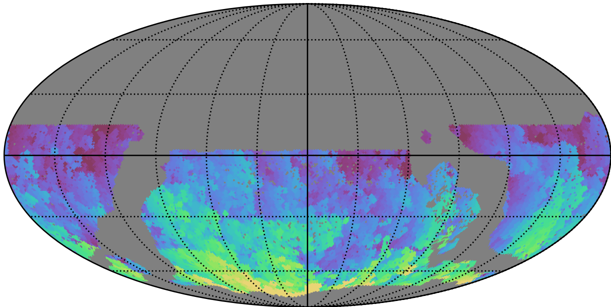
too_elab_r16_d3_griz_v3.4_10yrs WFD u band: Max HA
