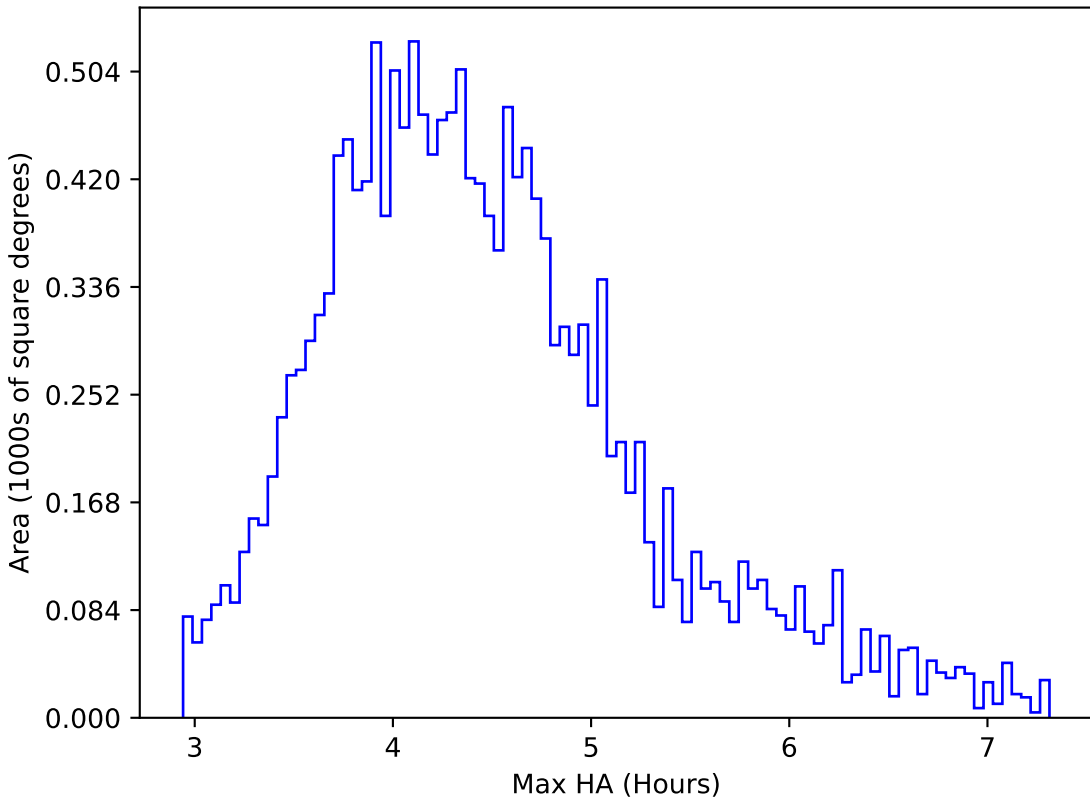
too_elab_r16_d3_griz_v3.4_10yrs WFD r band: Max HA
