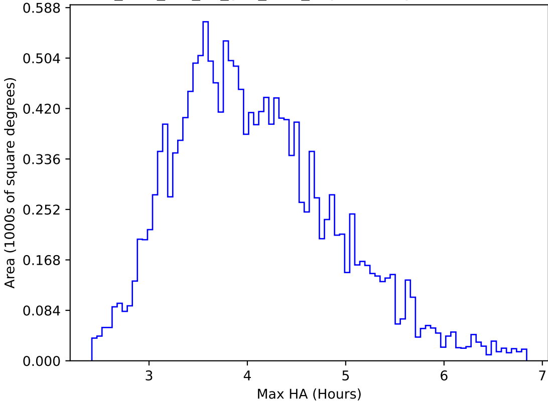
too_elab_r16_d3_griz_v3.4_10yrs WFD g band: Max HA
