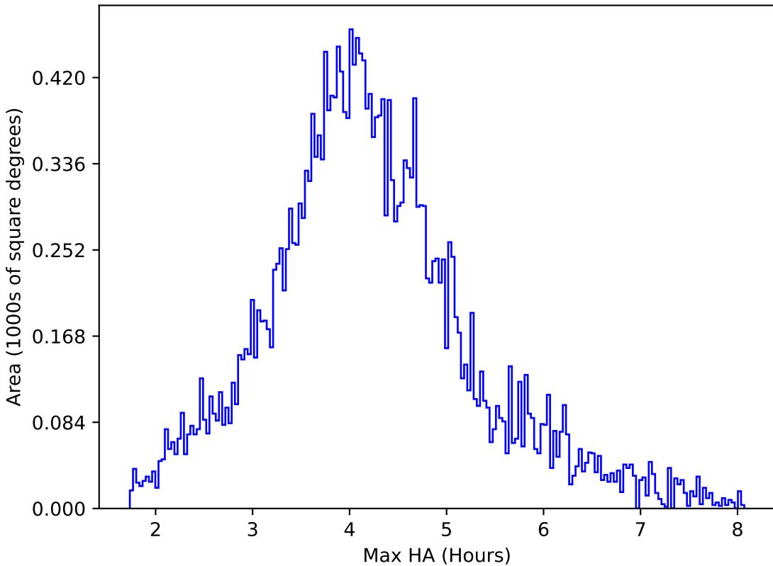
too_elab_r16_d3_griz_v3.4_10yrs All sky r band: Max HA
