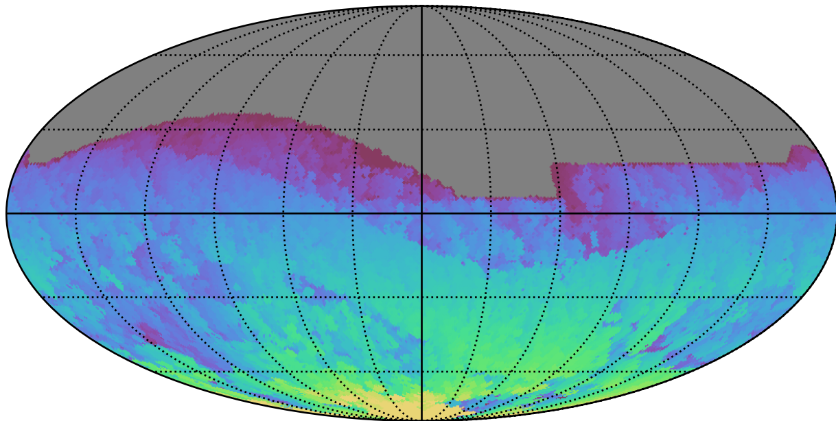
too_elab_r16_d3_griz_v3.4_10yrs All sky i band: Max HA
