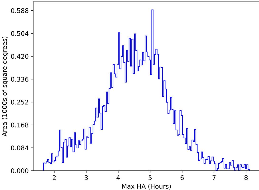
too_elab_r16_d3_griz_v3.4_10yrs All sky i band: Max HA
