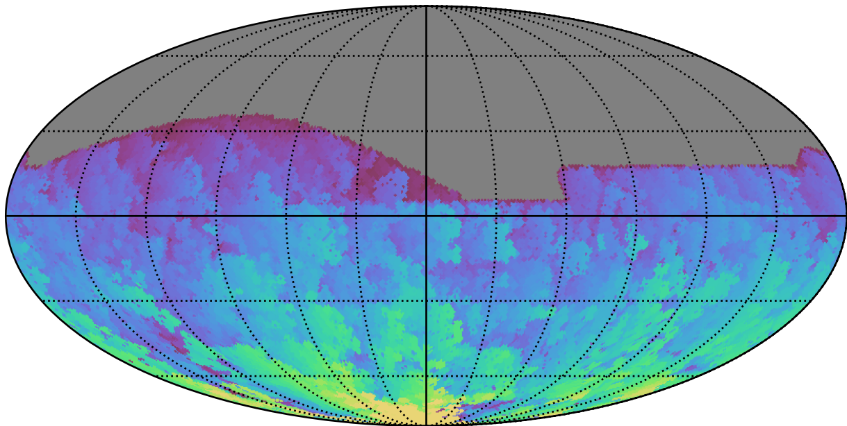
too_elab_r16_d3_griz_v3.4_10yrs All sky g band: Max HA
