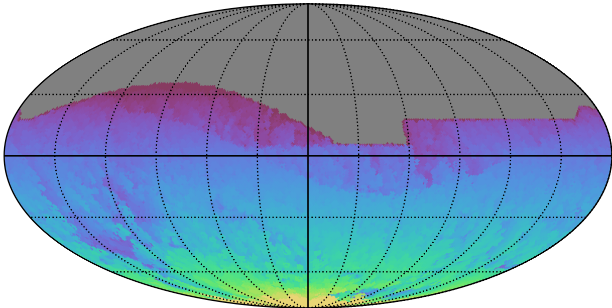
too_elab_r16_d3_griz_v3.4_10yrs All sky all bands: Max HA
