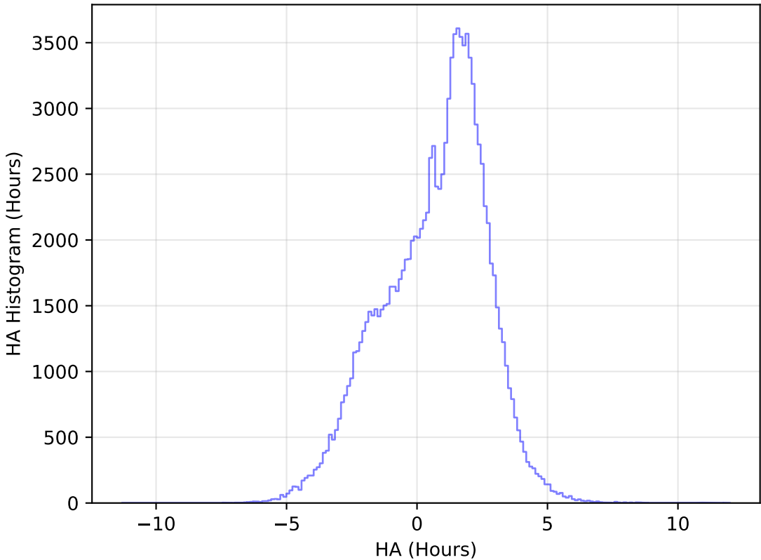
too_elab_r16_d3_griz_v3.4_10yrs WFD u band: HA Histogram
