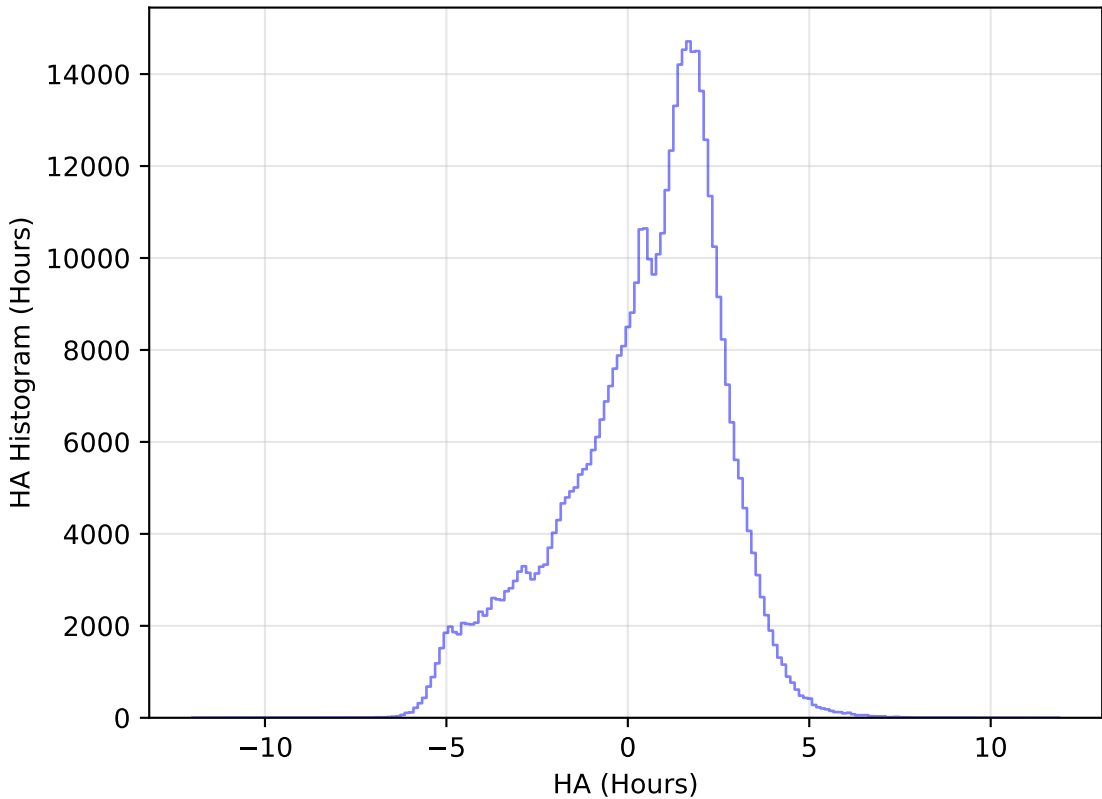
too_elab_r16_d3_griz_v3.4_10yrs WFD r band: HA Histogram
