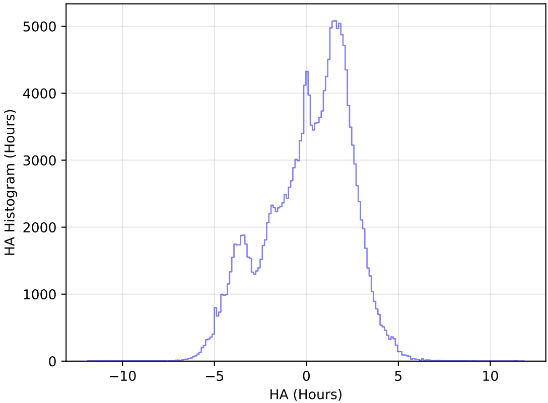
too_elab_r16_d3_griz_v3.4_10yrs WFD g band: HA Histogram
