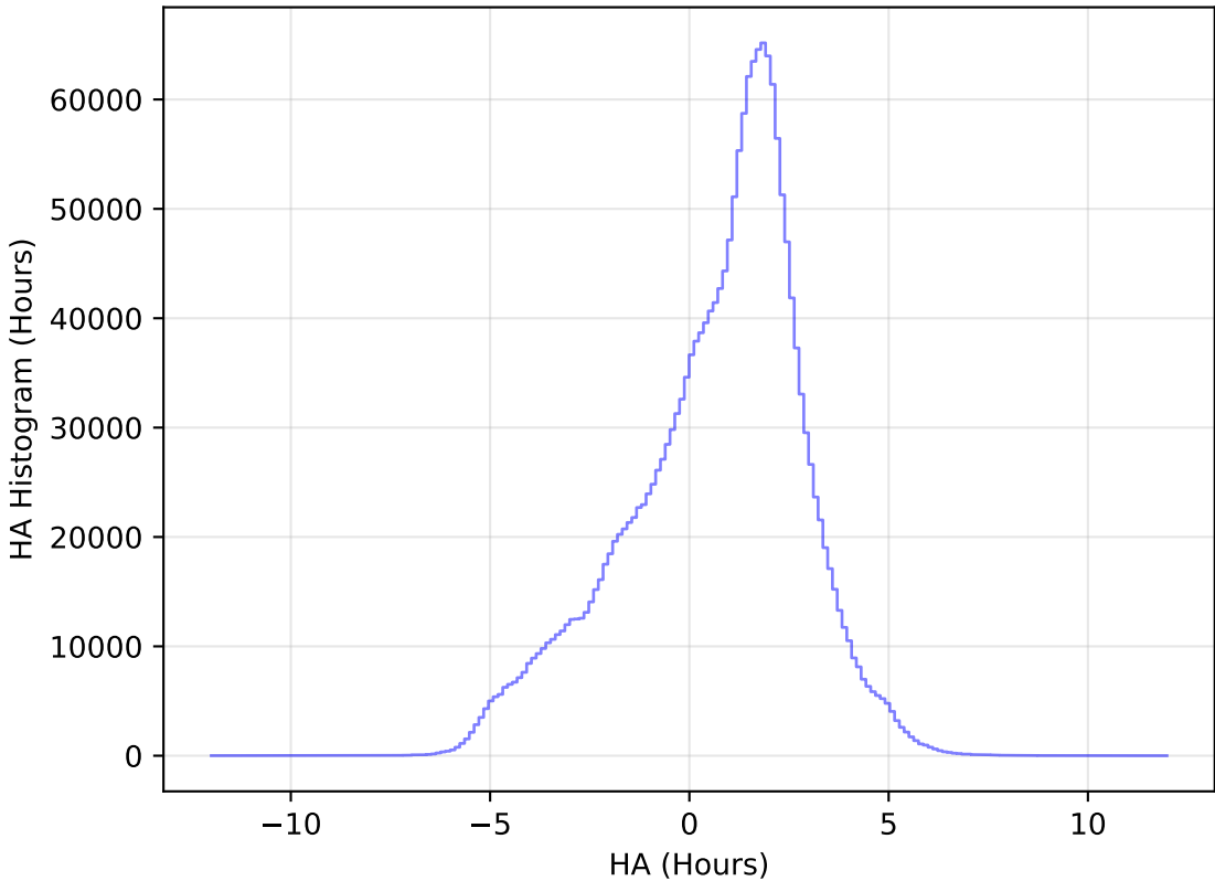
too_elab_r16_d3_griz_v3.4_10yrs WFD all bands: HA Histogram
