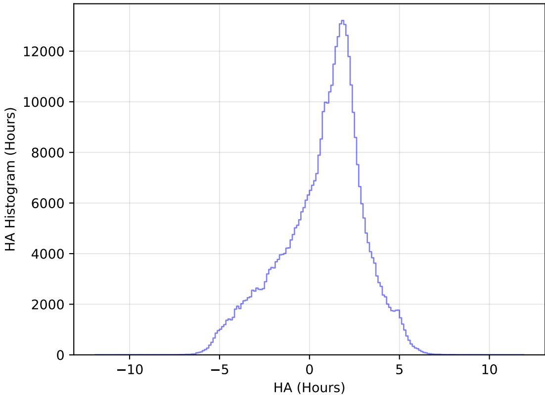
too_elab_r16_d3_griz_v3.4_10yrs All sky z band: HA Histogram
