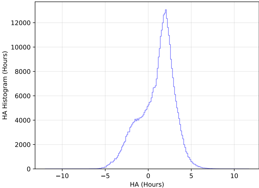
too_elab_r16_d3_griz_v3.4_10yrs All sky y band: HA Histogram
