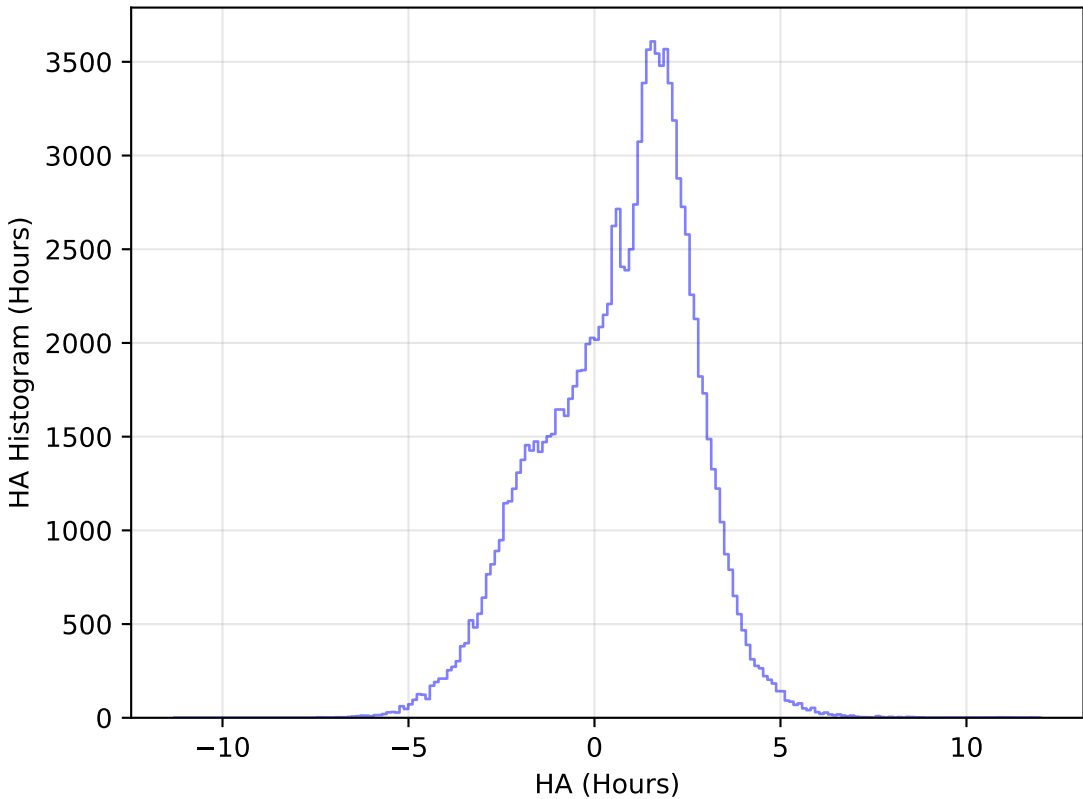
too_elab_r16_d3_griz_v3.4_10yrs All sky u band: HA Histogram
