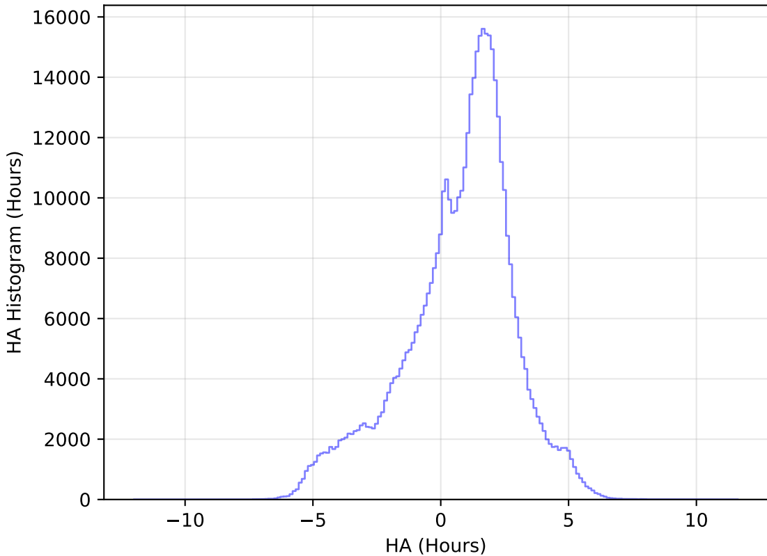
too_elab_r16_d3_griz_v3.4_10yrs All sky i band: HA Histogram
