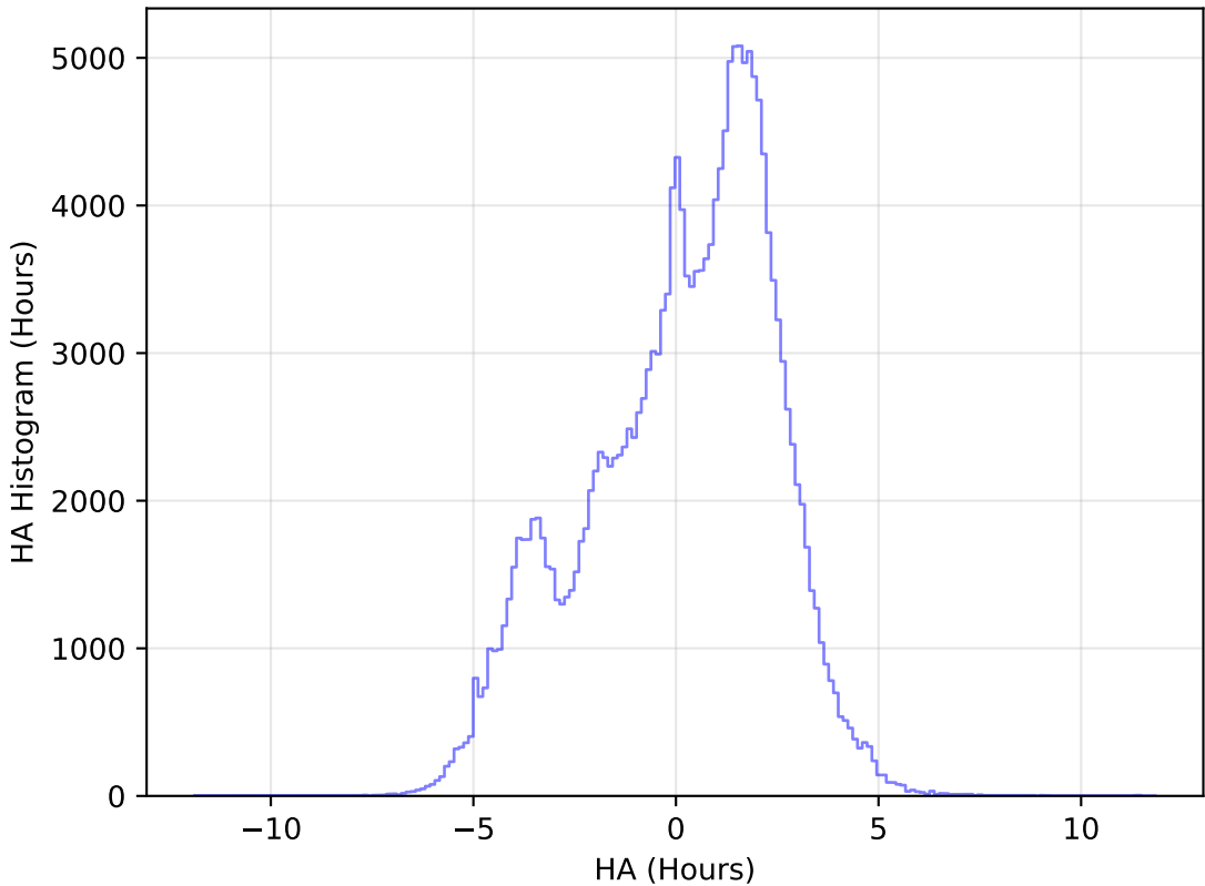
too_elab_r16_d3_griz_v3.4_10yrs All sky g band: HA Histogram
