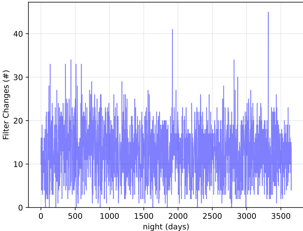
too_elab_r16_d3_griz_v3.4_10yrs Per Night: Filter Changes
