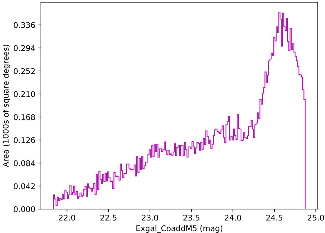
too_elab_r16_d3_griz_v3.4_10yrs Yr 3-4 z band: Exgal_CoaddM5
