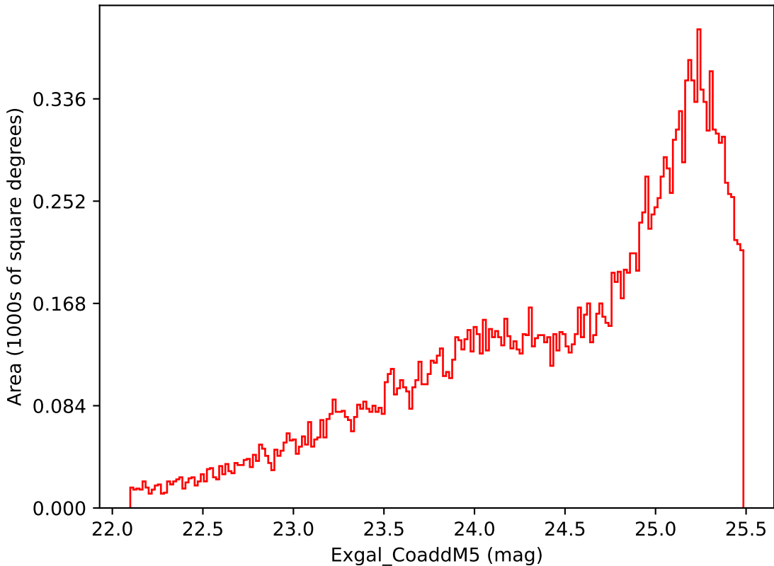
too_elab_r16_d3_griz_v3.4_10yrs Yr 3-4 i band: Exgal_CoaddM5
