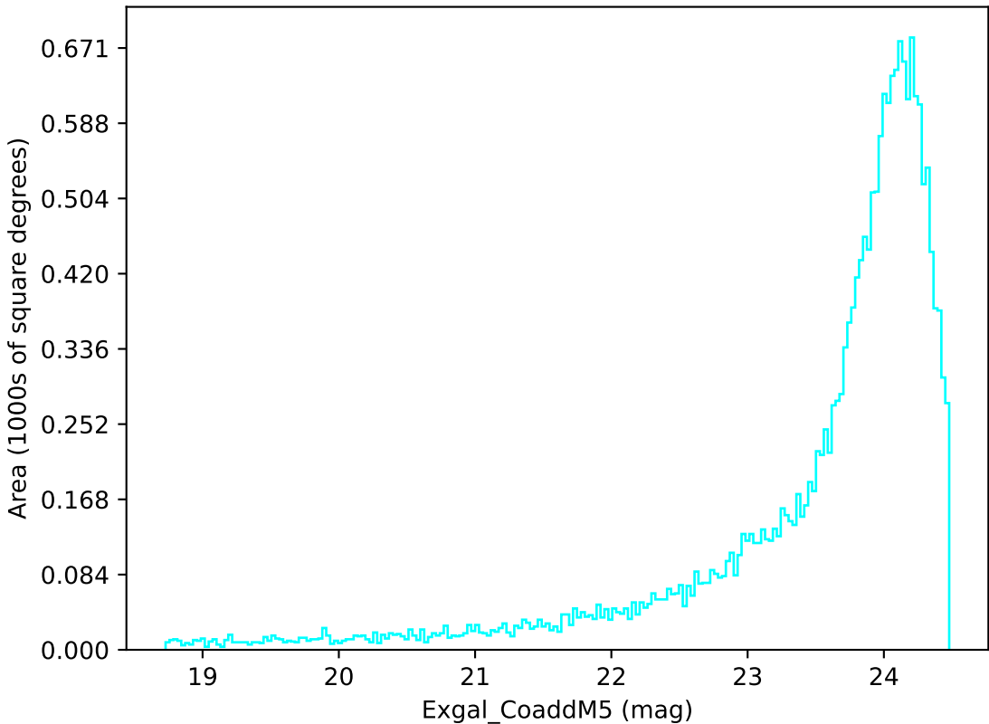
too_elab_r16_d3_griz_v3.4_10yrs Yr 1 u band: Exgal_CoaddM5
