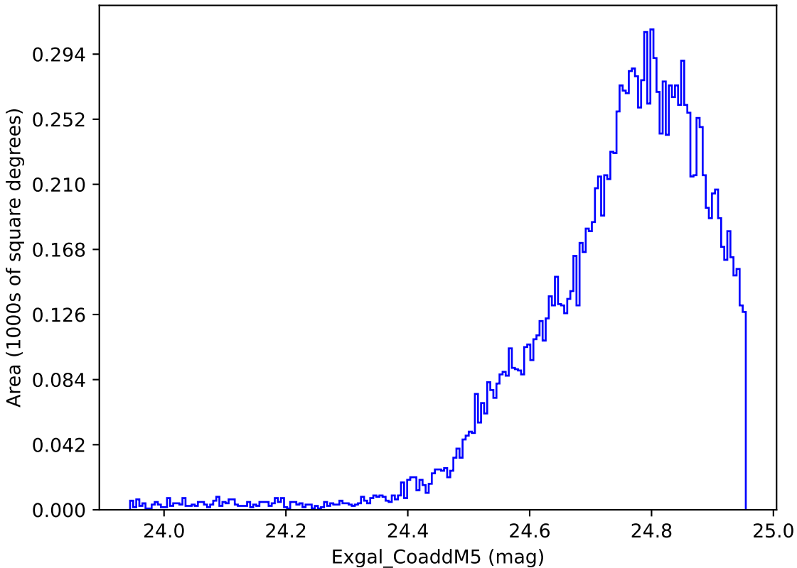
too_elab_r16_d3_griz_v3.4_10yrs WFD y band: Exgal_CoaddM5
