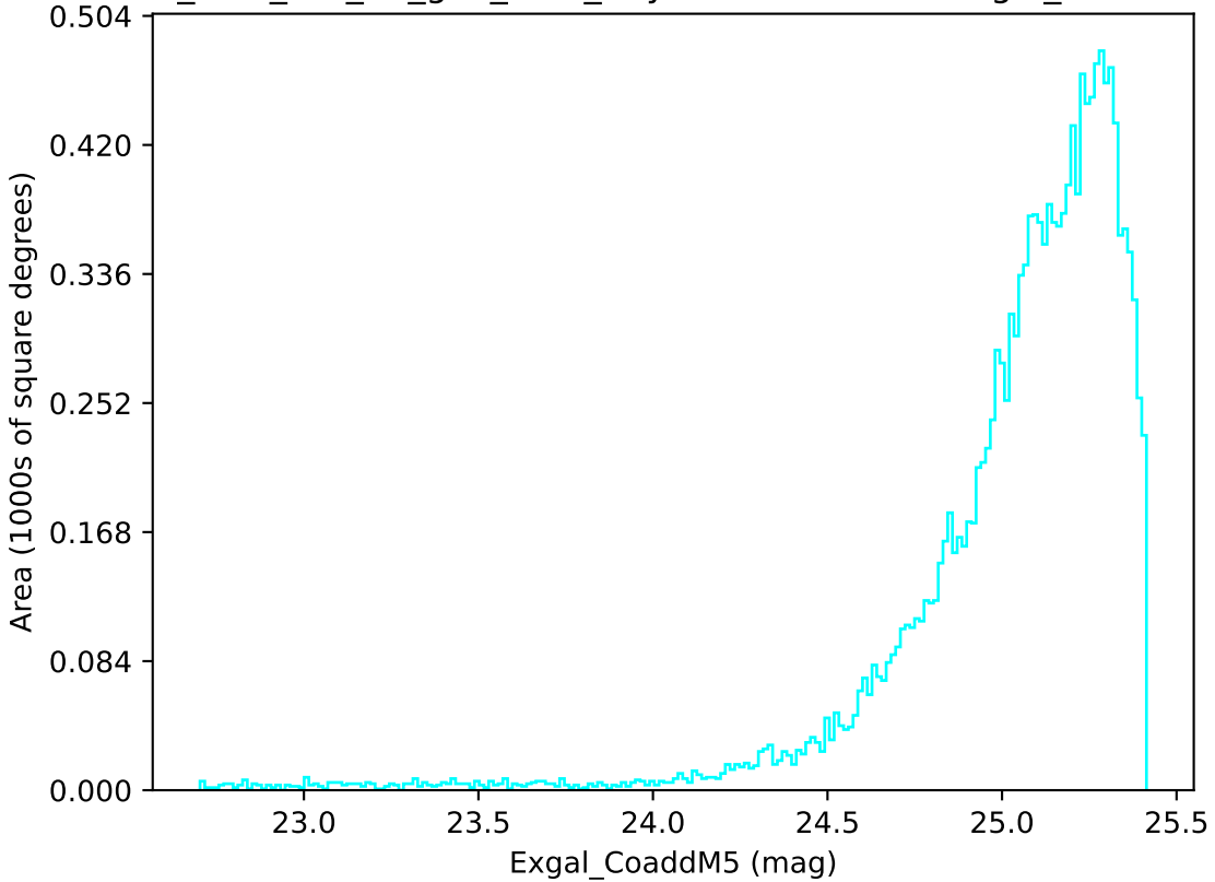
too_elab_r16_d3_griz_v3.4_10yrs WFD u band: Exgal_CoaddM5
