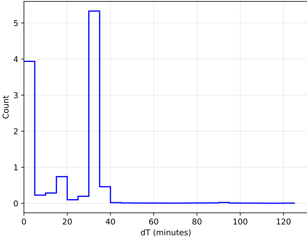
too_elab_r16_d3_griz_v3.4_10yrs WFD: DeltaT Histogram 1e6
