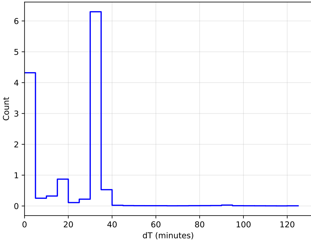
too_elab_r16_d3_griz_v3.4_10yrs All sky: DeltaT Histogram 1e6
