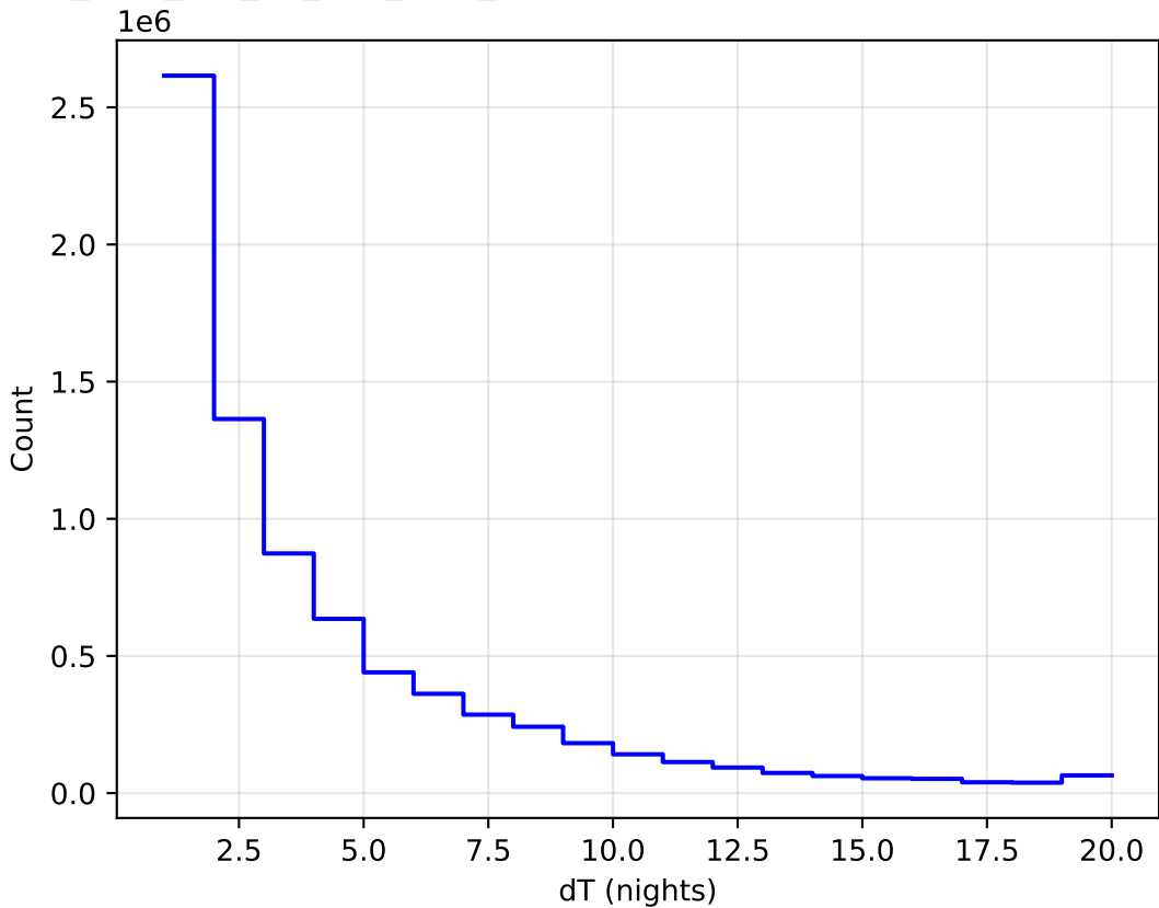
too_elab_r16_d3_griz_v3.4_10yrs WFD all bands: DeltaNight Histogram
