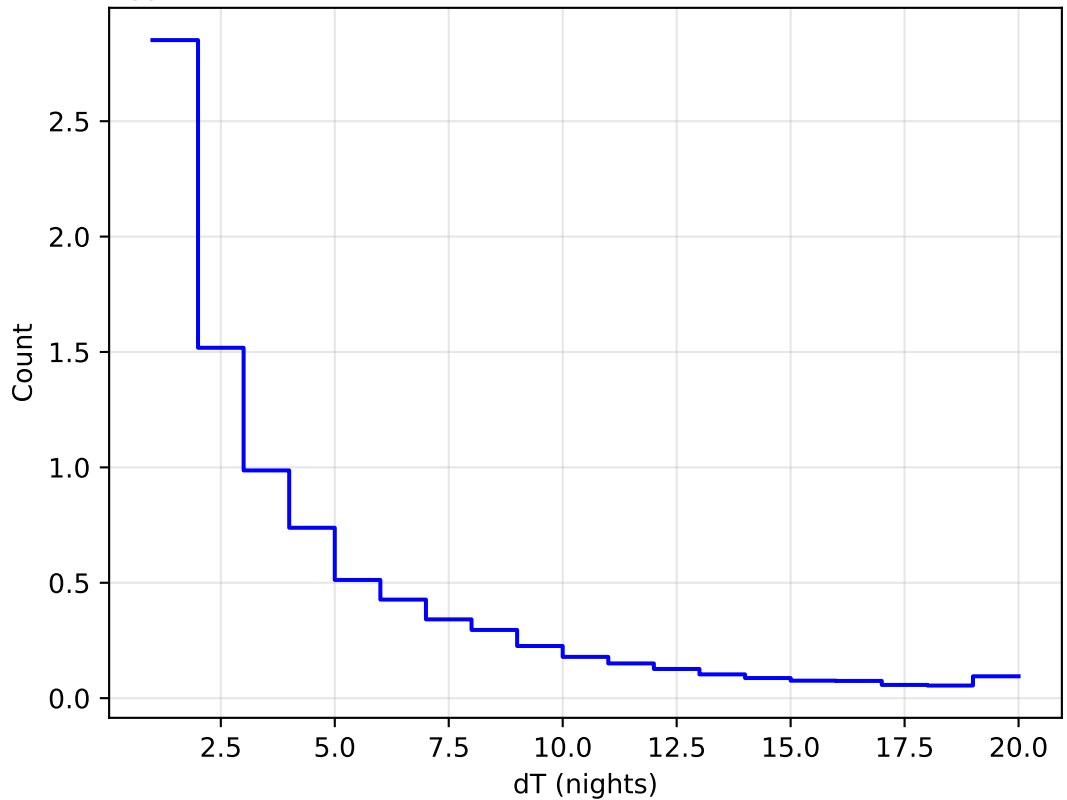
too_elab_r16_d3_griz_v3.4_10yrs All sky all bands: DeltaNight Histogram
