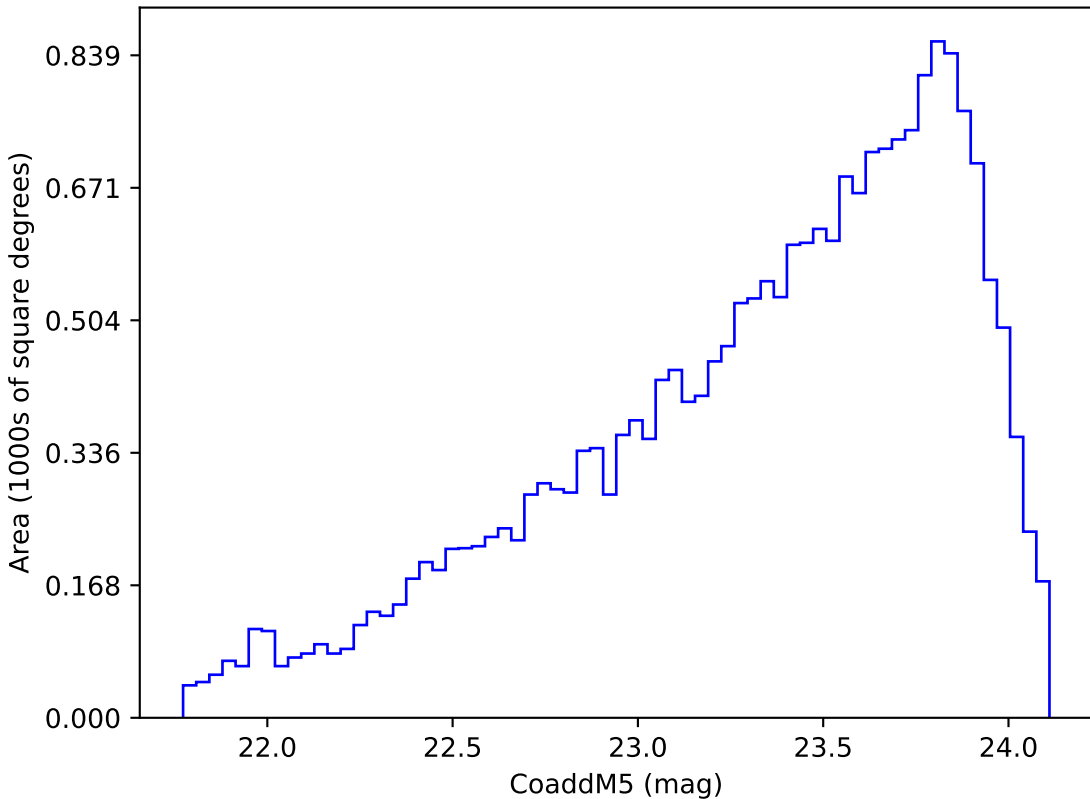
too_elab_r16_d3_griz_v3.4_10yrs Yr 3-4 y band: CoaddM5
